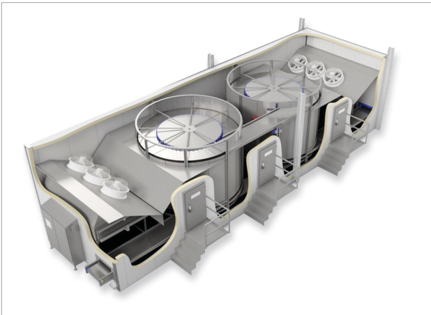
Double drum Spiral Freezer
